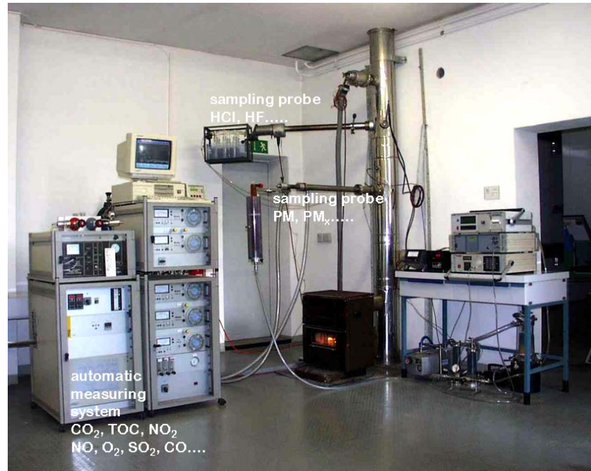
Fig. 1: Test arrangement household stove (brown coal briquette)
